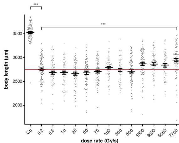
Figure 3 Effects of dose rate on zebrafish embryo length. Length of zebrafish embryos at 4 d postirradiation (5 days postfertilization; n = 57-88/point). **** = p < 10^{-4} , * = p < 0.05 . Abbreviation: ns = not significant.
